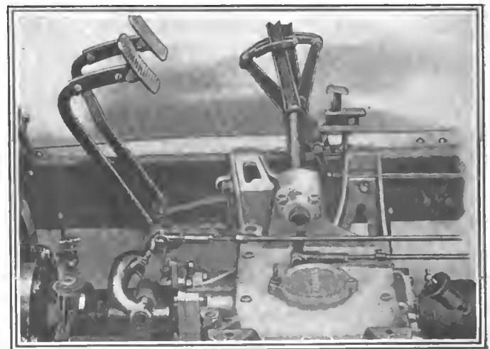
Fig. 4.—Gearbox and operating pedals on Premier
